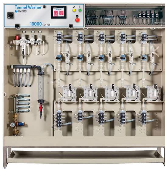
5-Channel Tunnel Configuration Model Number: HYDSPD0035M (Metric)
