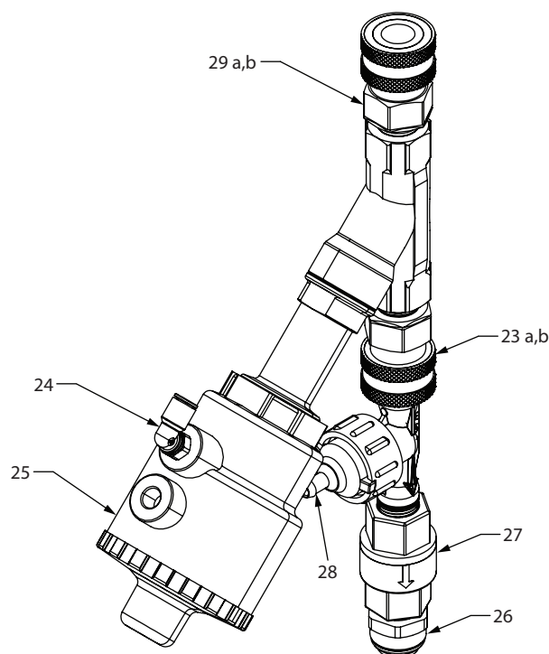
Seat Valve
